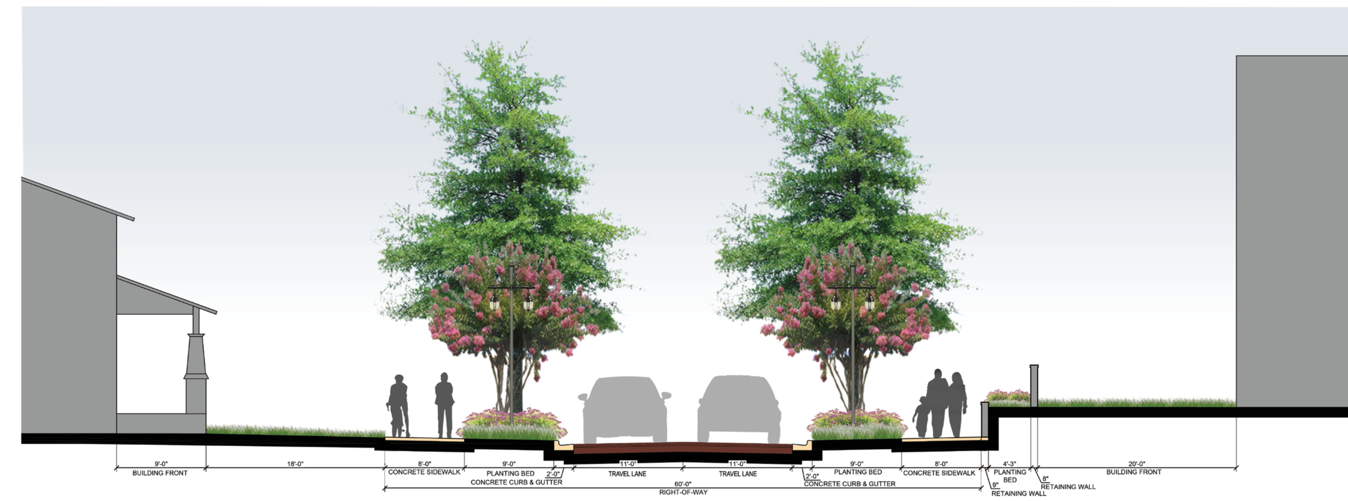
Proposed Section D'
